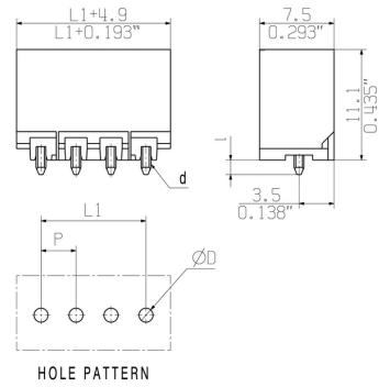
HOLE PATTERN
