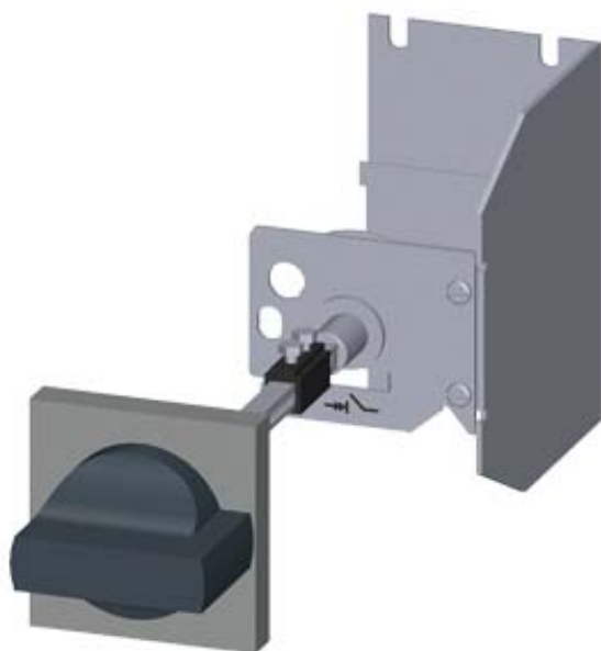
DOOR-COUPLING ROTARY OPERATING MECHANISM FOR CIRCUIT-BREAKERS SIZE S00/S0, HANDLE GRAY NEW DESIGN
