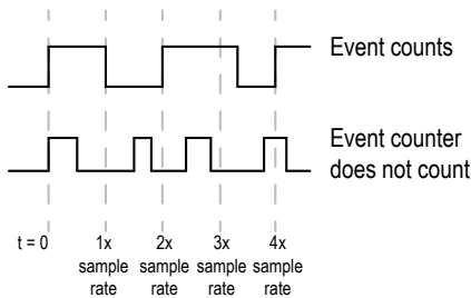
Figure 1. Event counter
