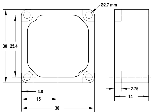
Figure 3. Stainless steel models
