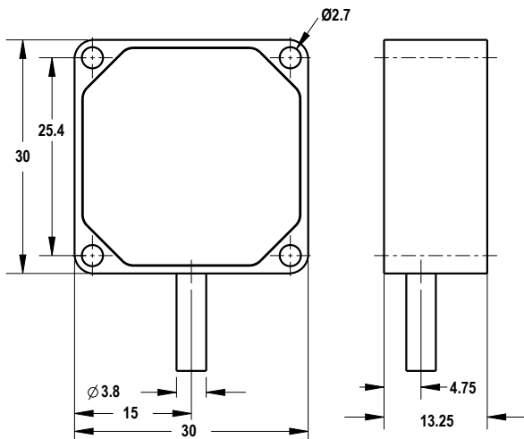
Figure 2. Aluminium model
