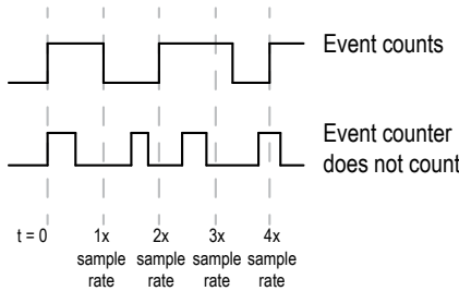
Figure 2. Event counter
