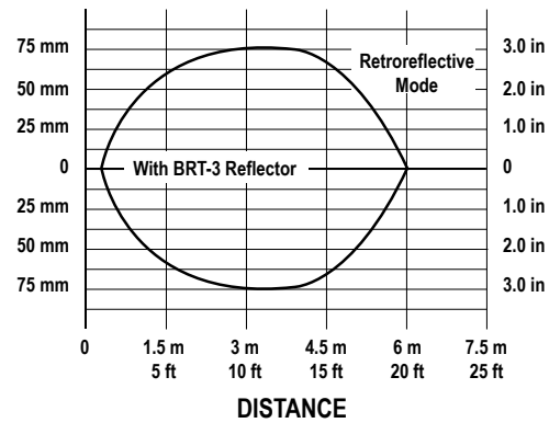
Figure 4. Beam Pattern
